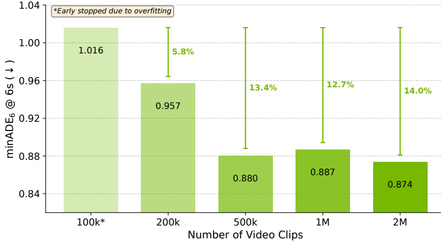
Figure 13: Impact of training data scale on open-loop driving performance. All models use the 0.5B architecture with identical hyperparameters and fixed total training steps. Models are evaluated on \mathcal{D}_{\text{overall}} held-out test set. *Early stopped due to overfitting.
