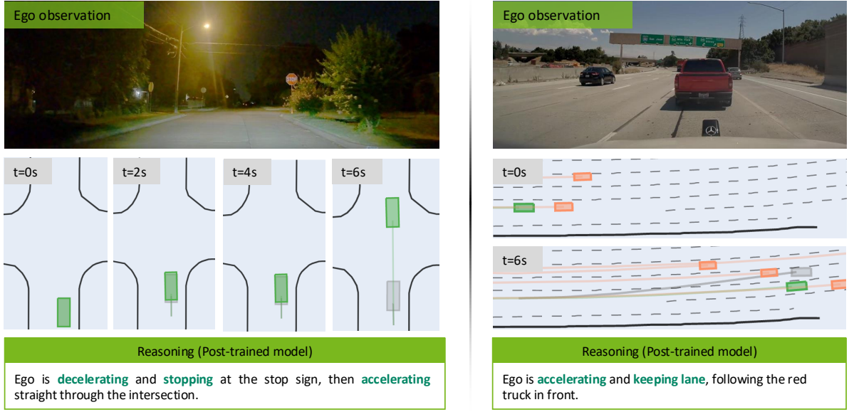
Figure 11: Post-training with the reasoning-action consistency reward improves motion fidelity. Grey motion denotes the most-likely rollout from the SFT-pretrained base model, and green motion denotes the most-likely rollout from the post-trained model. The orange motions denote the obstacles’ motion replay. Left: The base model (grey) stops halfway and fails to resume motion, even though its reasoning trace correctly instructs the ego vehicle to accelerate after stopping. The post-trained model (green) executes the full causal sequence: decelerating, stopping, and accelerating once the intersection is clear. Right: When the reasoning instructs the ego vehicle to follow a lead vehicle, the post-trained model’s generated motion maintains appropriate speed and lane position in accordance with its reasoning trace (“accelerating and keeping lane”), whereas the base model’s generated motion changes the lane, drifting from the intended plan.
