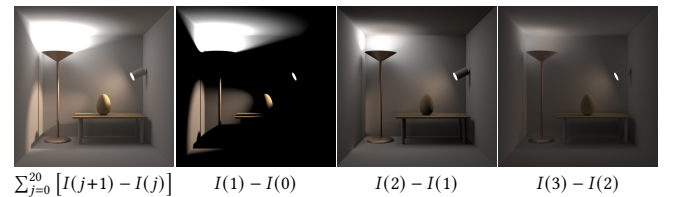
Fig. 2. Illustration of path tracing as an instance of Eq. (12). Each term in the summation is the difference in contribution between (j+1) - and j -length paths, simplifying to a sum over the contribution of various bounces.
