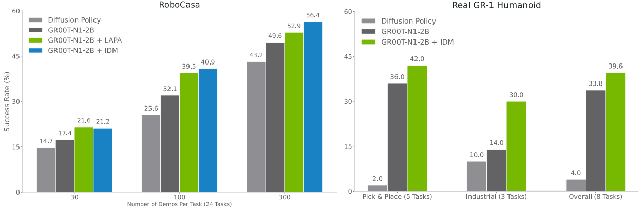
Figure 9: Average Success Rate (%) across 24 Tasks in simulation and 8 tasks in the real world. In the RoboCasa simulation, we show all post-training results using 30, 100, and 300 demonstrations per task. In the real world, we show results only on the low-data regime (10% of the demonstrations). We co-train with 3k neural trajectories per task for RoboCasa and 100 neural trajectories per task for real-world tasks. We explore using both latent and IDM-labeled actions in simulation and only IDM-labeled actions for the real robot.
