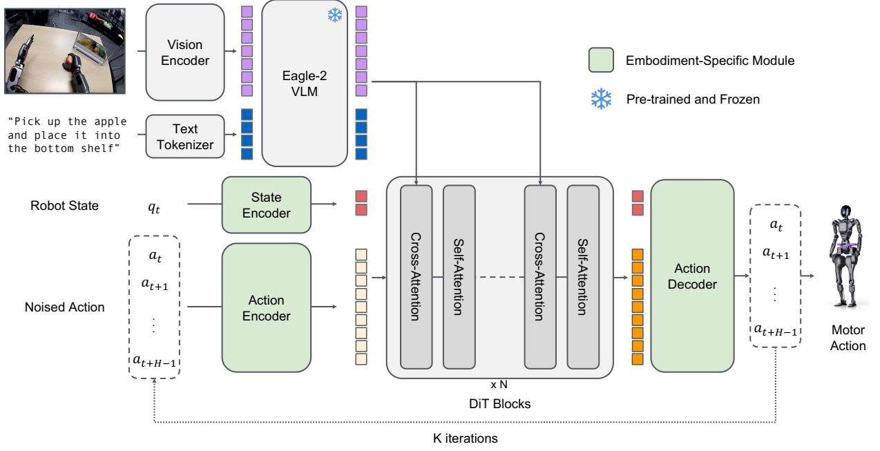
Figure 3: GR00T N1 Model Architecture. GR00T N1 is trained on a diverse set of embodiments ranging from single-arm robot arms to bimanual humanoid dexterous hands. To deal with different robot embodiment’s state observation and action, we use DiT blocks with an embodiment-aware state and action encoder to embed the robot’s state and action inputs. GR00T N1 model leverages latent embeddings of the Eagle-2 model to incorporate the robot’s visual observation and language instructions. The vision language tokens will then be fed into the DiT blocks through cross-attention layers.
