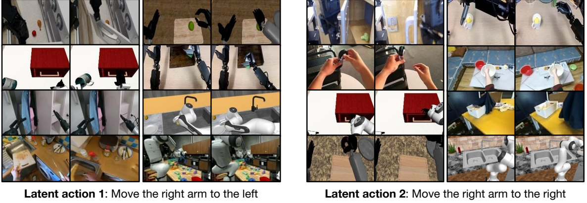
Figure 4: Latent Actions. We retrieve similar latent embeddings across various embodiments. The left image illustrates the latent action that corresponds to moving the right arm (or hand) to the left, while the right image illustrates the latent action that corresponds to moving the right arm (or hand) to the right. Note that this general latent action is not only consistent in different robot embodiments, but also in human embodiment.
