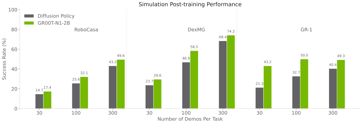
Figure 10: Average policy success rate on simulated manipulation tasks with varying numbers of demonstrations.
